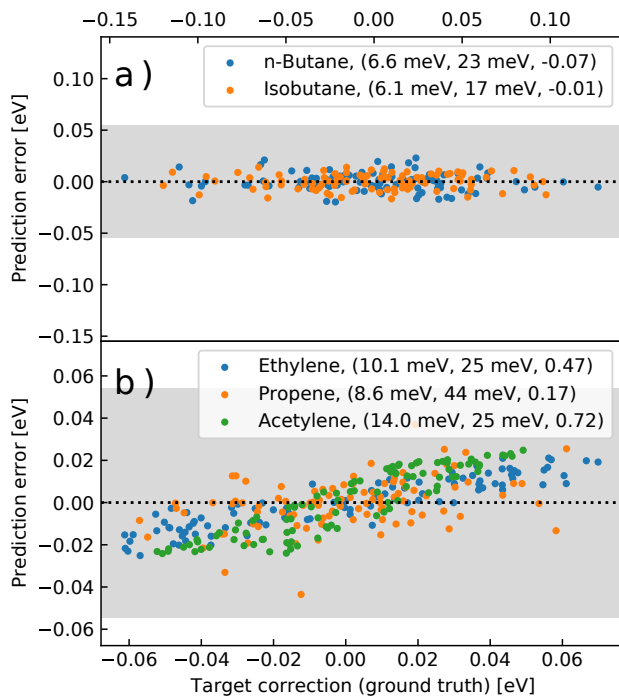
FIG. 4. Residuals for transferability task on small alkanes. Values on the x-axis, the target corrections, correspond to the errors in total energy of PBE compared to the reference method CCSD(T). Prediction errors on the y-axis are defined as the errors of NeuralXC optimized on ethane and propane with respect to CCSD(T). Shaded area corresponds to an error of \pm 2 mH, the threshold chosen by Cheng et al. [26]. Values in parentheses correspond to (Mean absolute error, Maximum absolute error, R^2 for the residuals).
