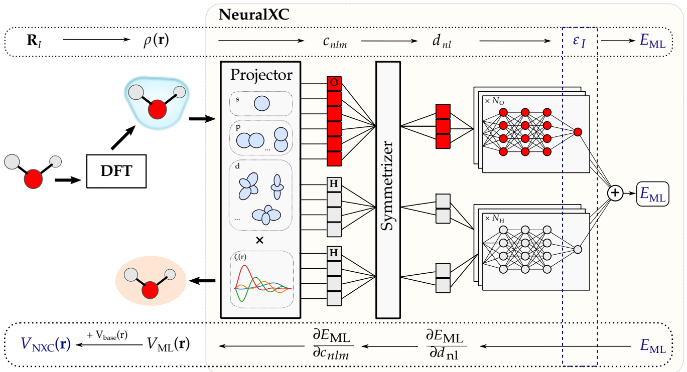
FIG. 1. Implementation of NeuralXC. Starting from the electron density in real-space, obtained with a converged DFT calculation (using the baseline functional E_{base} ), the projector maps this density to a set of descriptors c_{nlm} . The symmetrizer creates rotationally invariant versions of these descriptors d_{nl} , which, after preprocessing (not depicted here), are passed through a Behler-Parrinello type neural network architecture. By using the same network for descriptors of a given atomic species, we ensure permutation invariance. Once the energy E_{ML} is obtained, its derivative can be backpropagated using the chain rule to obtain the machine learned potential V_{ML} . V_{ML} is added back to the baseline potential V_{base} = \delta E_{base} / \delta n(\mathbf{r}) , to create the full V_{NXC}(\mathbf{r}) , which can be used in subsequent self-consistent calculations.
