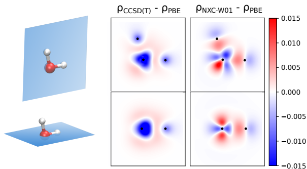
FIG. 7. Electron density of water. Comparison of the difference in electron density between CCSD(T) and PBE and NXC-W01 and PBE for a water molecule in its experimental equilibrium geometry. Two dimensional cuts either correspond to high-symmetry planes or planes containing a significant number of atoms and are indicated by blue surfaces in the molecule depictions adjacent to the density plots. Black dots inside the density plots indicate the positions of in-plane atoms. Atoms are color-coded with red corresponding to oxygen and white to hydrogen. Color scale is in units of e \cdot \text{Bohr}^{-3} .
