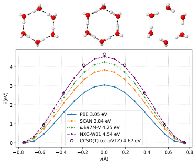
FIG. 6. Coordinated proton transfer in a water hexamer ring. The reaction coordinate is defined as \nu = d(O-H) - d(O'-H) , where O, O' , where O, O' are the two Oxygen atoms involved in the H-bond and H is the transferred proton. Energy values shown in inset correspond to barrier heights.
