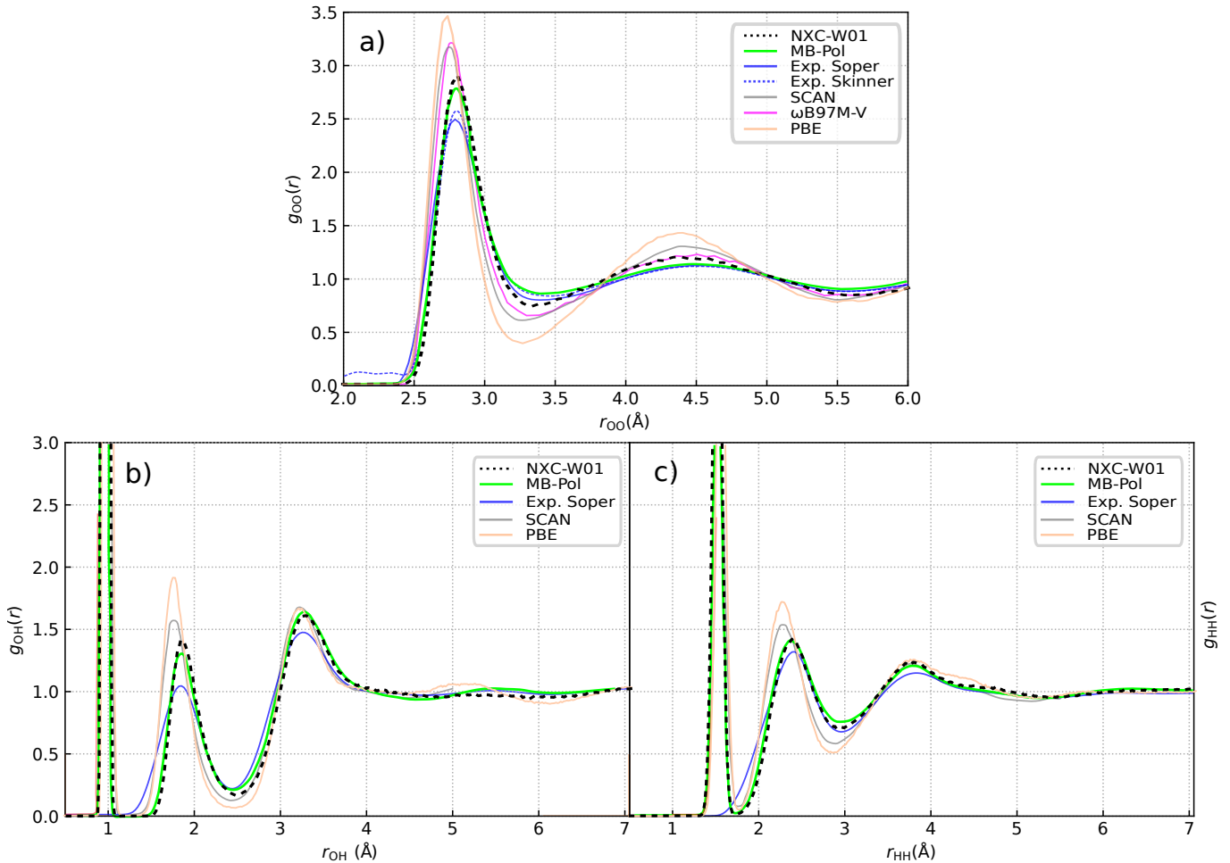
FIG. 5. Radial distribution functions (RDFs). The RDFs obtained from Born-Oppenheimer molecular dynamics simulations of 96 water molecules in a periodic box at experimental density and 300 K using PBE and NXC-W01 as functionals are compared to experimental results by Skinner et al. [28] and Soper [29] as well as MB-Pol results taken from Ref. [11] and Born Oppenheimer MD simulations using SCAN by Wiktor et al. [30] and \omega B97M-V by Yao et al. [31].
